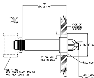
RECESSED HORIZONTAL SIDEWALL
