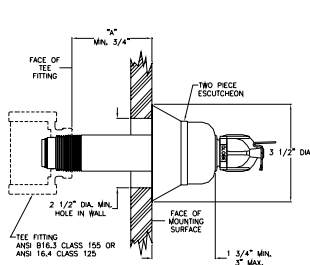
EXTENDED HORIZONTAL SIDEWALL
