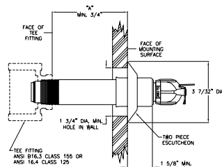
SLEEVE & SKIRT HORIZONTAL SIDEWALL
