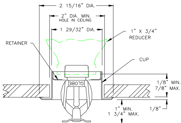
CROSS SECTION
